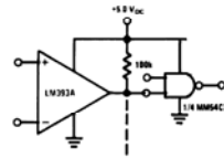
Driving CMOS
