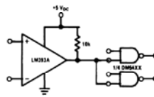
Driving TTL
