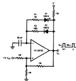
Pulse Generator
