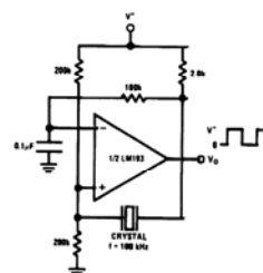
Crystal Controlled Oscillator
