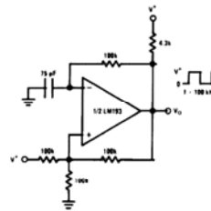
Squarewave Oscillator
