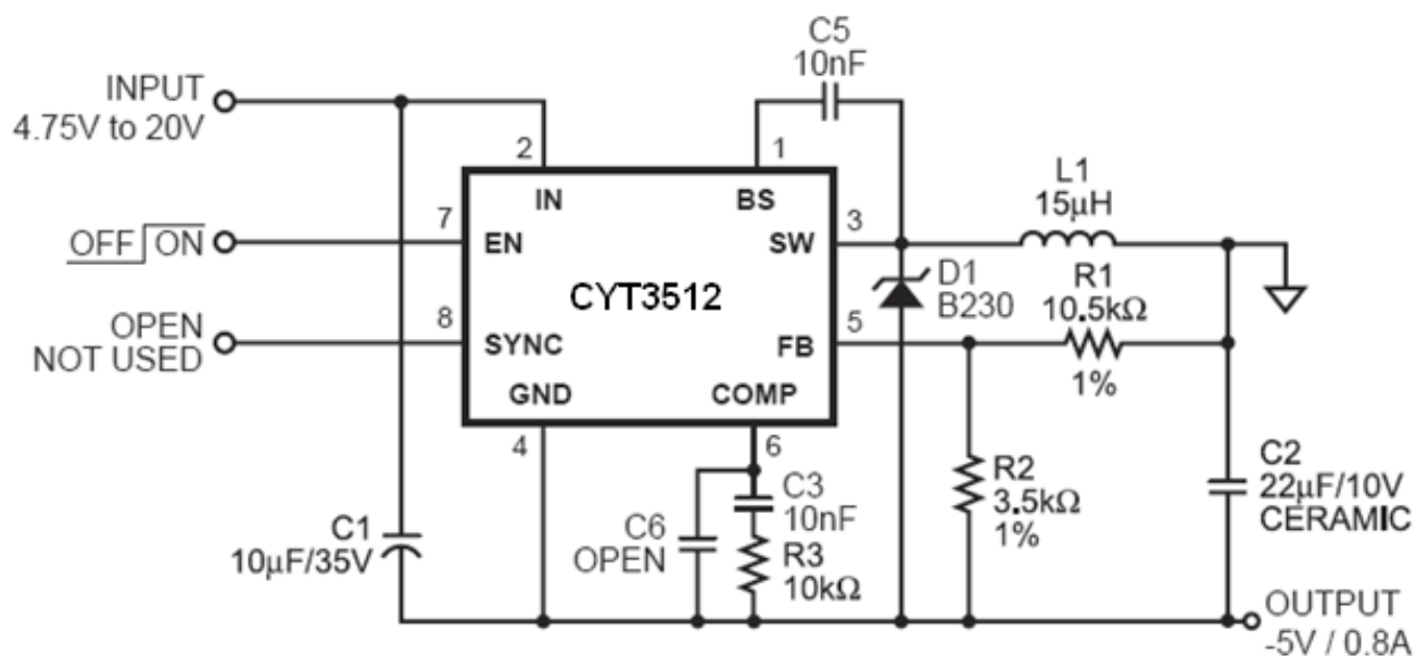
Figure 3—Application Circuit for -5V Supply
